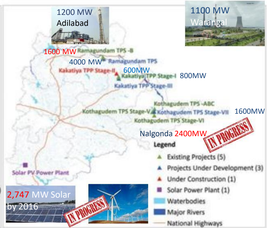
Spatial Distribution of Thermal & Solar Power Plants
