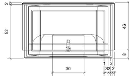
Front View 1:1
