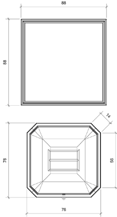
Plan View 1:1
