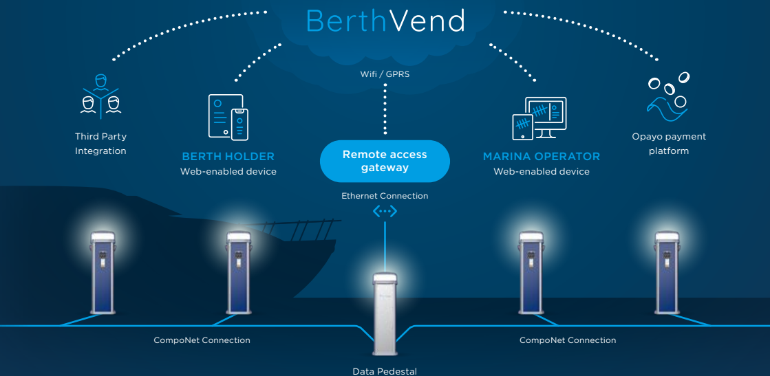
A TYPICAL BERTHVEND WIRED INSTALLATION EXAMPLE
