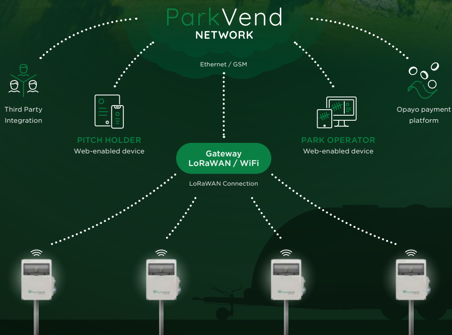
A TYPICAL PARKVEND NETWORK WIRELESS INSTALLATION EXAMPLE
