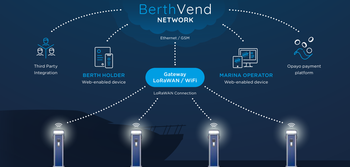
A TYPICAL BERTHVEND NETWORK WIRELESS INSTALLATION EXAMPLE
