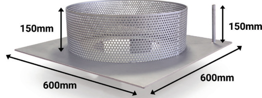
Underfloor Cooling
