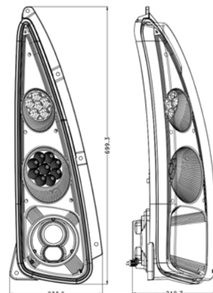
400073 | OE Ref: 87529731 - LED HEADLIGHT - LEFT / RIGHT NEW HOLLAND TG T8000 SERIES
