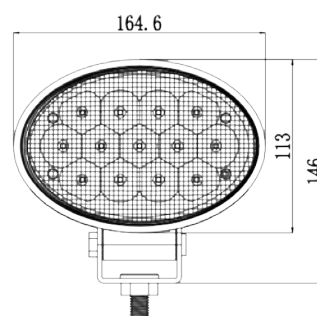
600000 OVAL 12V WORK LIGHT - MASSEY FERGUSON 5400 5600 6400 6600 7400 7600 8400 SERIES
