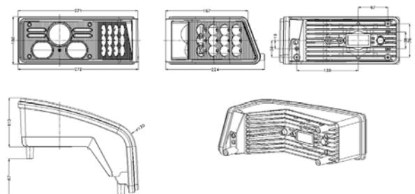
400070 | OE Ref: 178318A1 - LED HEADLIGHT - LEFT AND RIGHT CASE SERIES
