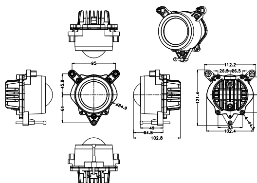
57233LED LH - LED PROJECTOR HEADLIGHT LEFT JOHN DEERE 5000 5003 5004 5D 5E SERIES
