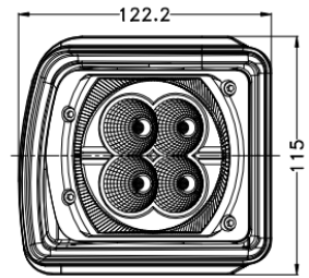
500100 | OE Ref: AL172568 LED WORK LIGHT - LEFT AND RIGHT JOHN DEERE 5M 5020 6020 6030 7030 SERIES
