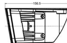
400072 | OE Ref: 279221A1 - LED AMBER CORNER LIGHT - WORK LIGHT LEFT AND RIGHT CASE MX SERIES
