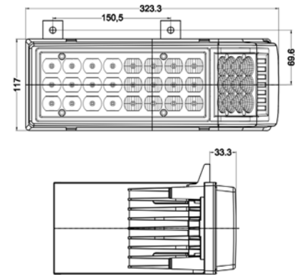
400071 | OE Ref: 86514347 - LED HEAD LAMP - HI/LOW BEAM AND SIDE BEAM NEW HOLLAND 70 SERIES
