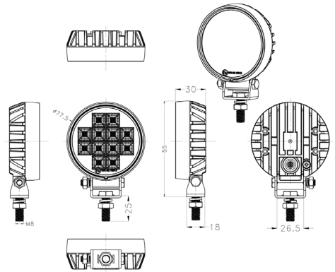
100069 - LED WORKLIGHT - 3 INCH ROUND 12W 900 UTILITY HIGH INTENSITY LUMENS
