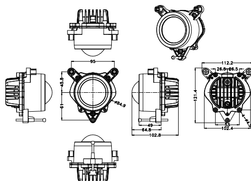
57233LED RH - LED PROJECTOR HEADLIGHT RIGHT JOHN DEERE 5000 5003 5004 5D 5E SERIES
