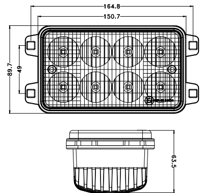
499992 | OE Ref: LVA14946 RECTANGULAR HEADLIGHT - JOHN DEERE 2000 3020 4000 6003 6E 6M SERIES
