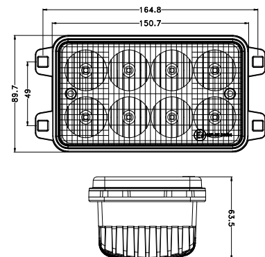
499993 | OE Ref: RE135400 LED HEADLIGHT - JOHN DEERE 5000 5003 5005 5010 5020 SERIES
