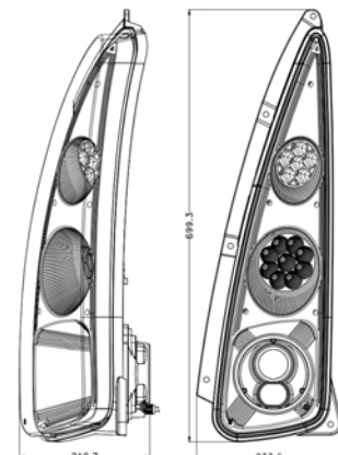
400072 | OE Ref: 279221A1 - LED AMBER CORNER LIGHT - WORK LIGHT LEFT AND RIGHT CASE MX SERIES
