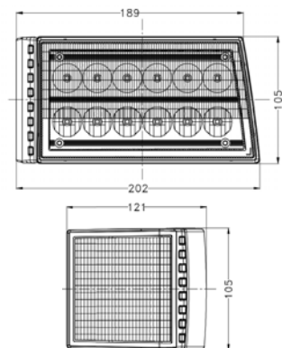
400067 | OE Ref: 91971C2 - LED HEADLIGHT - LEFT AND RIGHT CASE MAGNUM SERIES
