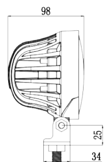
600000 OVAL 12V WORK LIGHT - MASSEY FERGUSON 5400 5600 6400 6600 7400 7600 8400 SERIES
