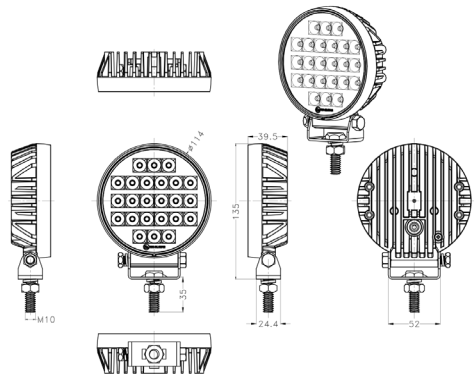
100070 - LED WORKLIGHT - 4 INCH ROUND 24W UTILITY HIGH INTENSITY 1,800 LUMENS
