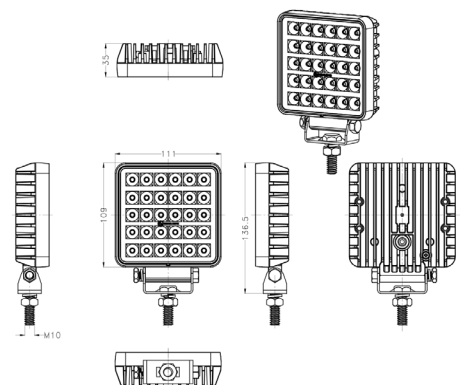
100074 - LED WORKLIGHT - 4 INCH SQUARE 30W UTILITY HIGH INTENSITY 2,200 LUMENS
