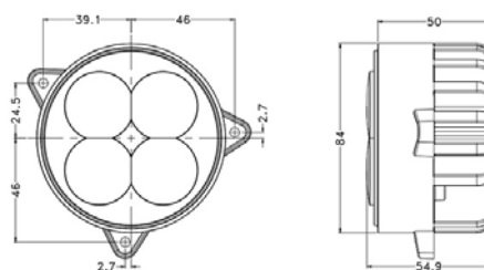
58049LED | OE Ref: AL209455 - LED WORKLIGHT - JOHN DEERE 6M 6R 6RC SERIES
