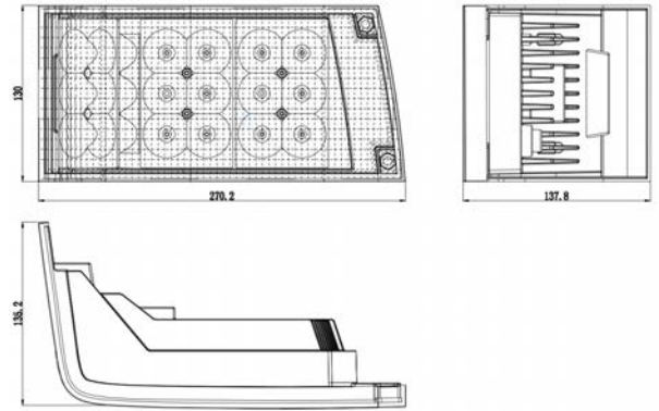
400067 | OE Ref: 91971C2 - LED HEADLIGHT - LEFT AND RIGHT CASE MAGNUM SERIES
