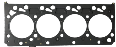
CYLINDER HEAD GASKET 400475 | OE Ref: 47667973 New Holland T5 T6 Series
