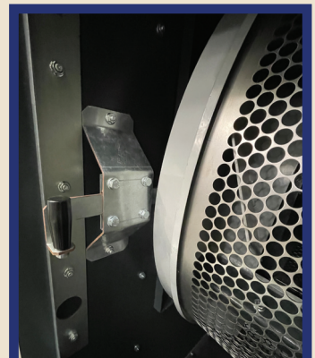
Cylinder Locking Latch
