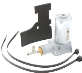
COMPRESSOR 24V Part no. 11996198
