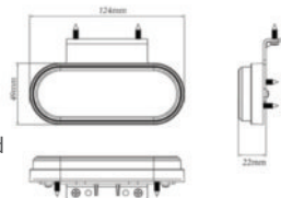
LUKA652 LED Marker Light - Oval Red Reflector within the light Zero Radio interference Top Mount Bracket included
