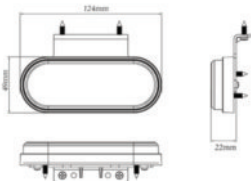
LUKA650 LED Marker Light - Oval White Reflector within the light Zero Radio interference Top Mount Bracket included
