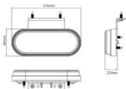
LUKA651 LED Marker Light - Oval Amber Reflector within the light Zero Radio interference Top Mount Bracket included
