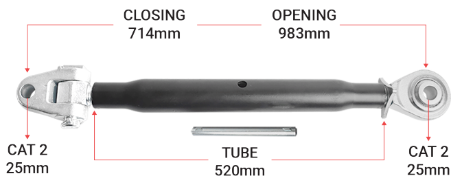
TOP LINK CAT 2 KB22380 | OE Ref: S99505 2 Knuckle Ball 380mm Heavy Duty
