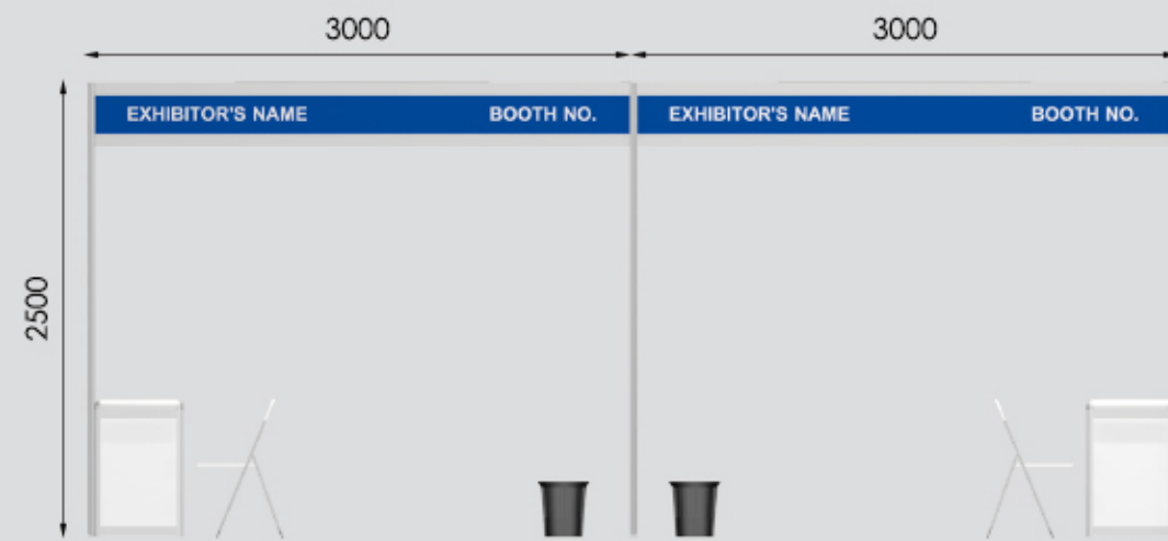
LEFT ELEVATION
