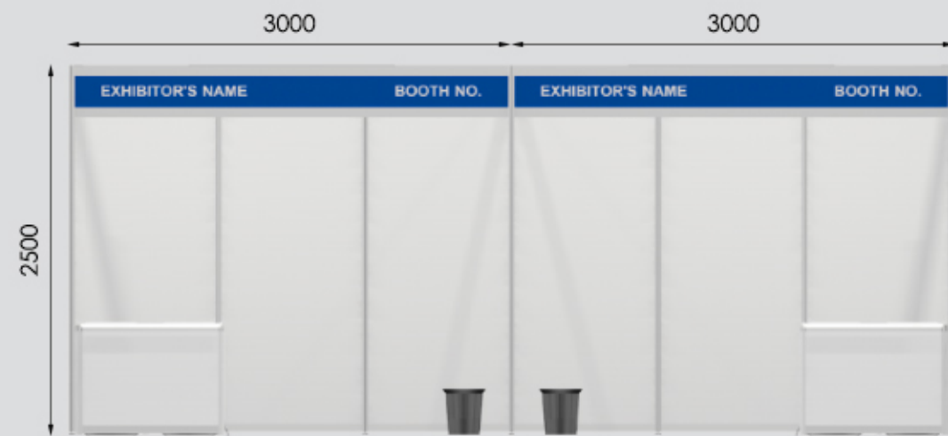
FRONT ELEVATION
