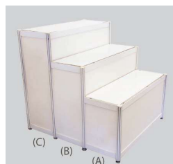
S11 3-Tier Display Counter (A) 1000L x 310W x 500H (B) 1000L x 310W x 750H (C) 1000L x 310W x 1000H
