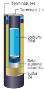
Battery Cell
