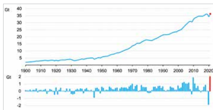
Figure 7: Total CO 2 emissions from energy combustion and industrial processes and their annual change, 1900–2021 Source: Global Energy Review: CO 2 Emissions in 2021
