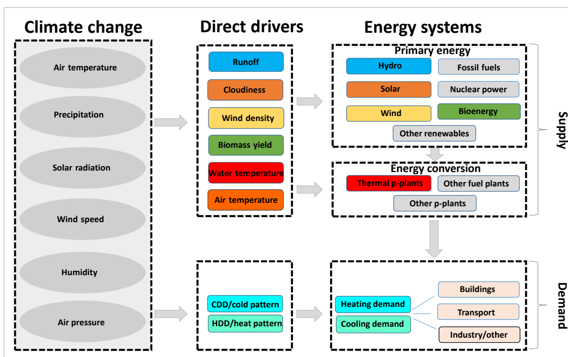
Figure 5: Conceptual framework of climate impacts on the energy sector. CDD – cooling degree days; HDD – heating degree days. Source: Impacts of Climate Change on Energy Systems in Global and Regional Scenarios
