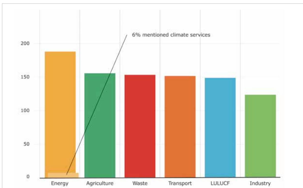
Figure 10: Sectors covered by NDC mitigation targets, in number of Parties from 2016 to March 2022. LULUCF – land use, land-use change and forestry.
