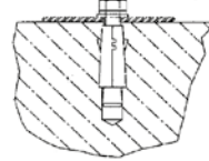
Fixing with screw anchors
