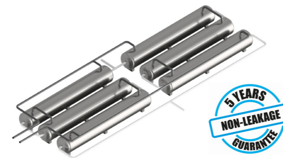
The Aalborg CSP header-and-coil oil-to-salt heat exchanger
