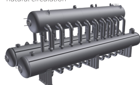
Steam Generation System configuration 3 evaporator and steam drum with natural circulation
