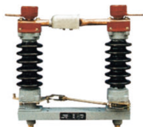
GW4-40.5 outdoor high voltage disconnecting switch
