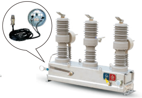
ZW32 intelligent HV vacuum circuit breaker
