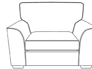
Lovechair H:98 x W:141.5 x D:96 (cm) x1 Small Scatter
