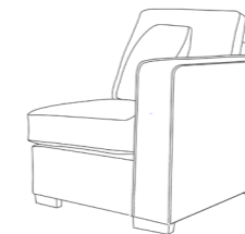
Right Hand Arm Unit H:94 x W:112 x D:99 (cm) x1 Small Scatter x1 Arm Cushions
