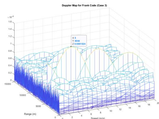
Fig. 8. Doppler Map for Frank Code
