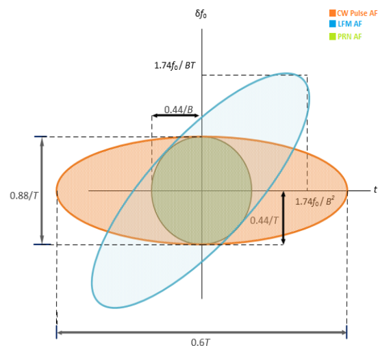
Fig. 1. Ambiguity Function (AF) of CW, FM and PRN waveforms
