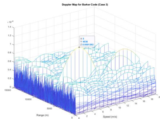
Fig. 7. Doppler Map for Barker Code
