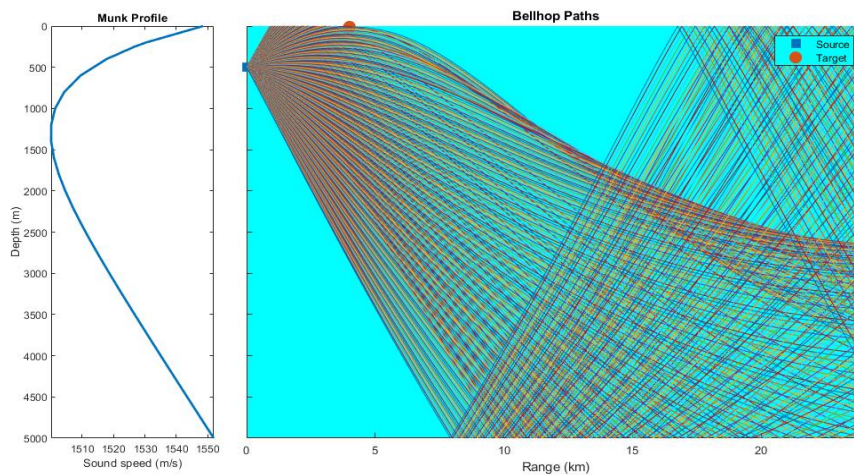
Fig. 4. Bellhop Ray Trace for Case 3
