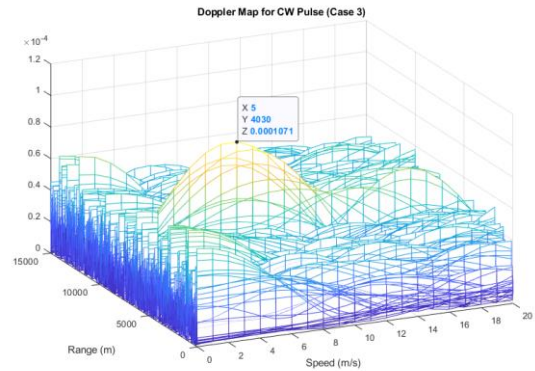
Fig. 5. Doppler Map for CW Pulse
