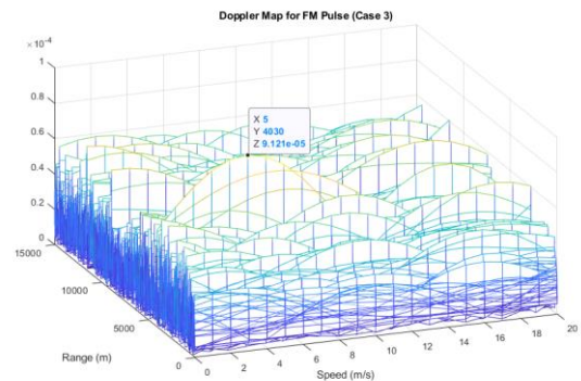
Fig. 6. Doppler Map for FM Pulse
