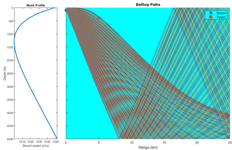
Fig. 3. Bellhop Ray Trace for Case 1 and Case 2
