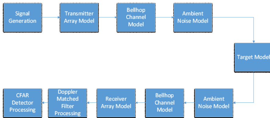
Fig. 2. Sonar Simulation Model
