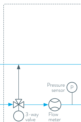
LAUDA MID 80 Flow control unit
