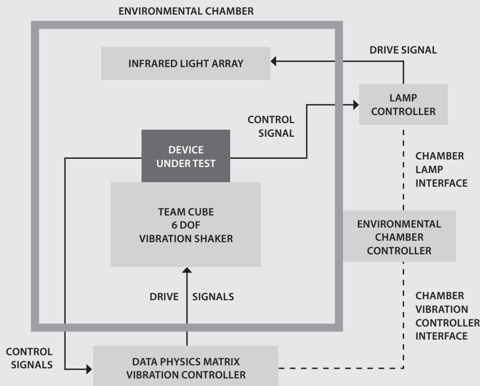
Figure 2. Integration of Temperature, Vibration, and Radiation Testing
