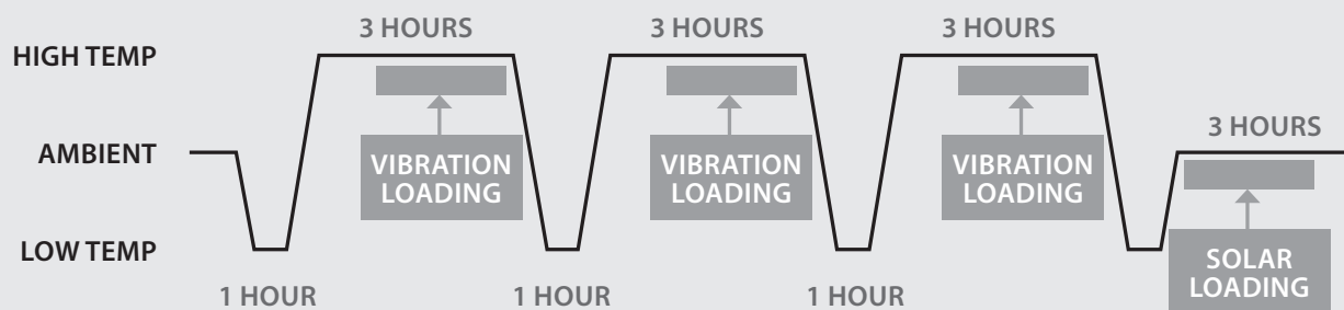
Figure 4. Example System Test Profile
