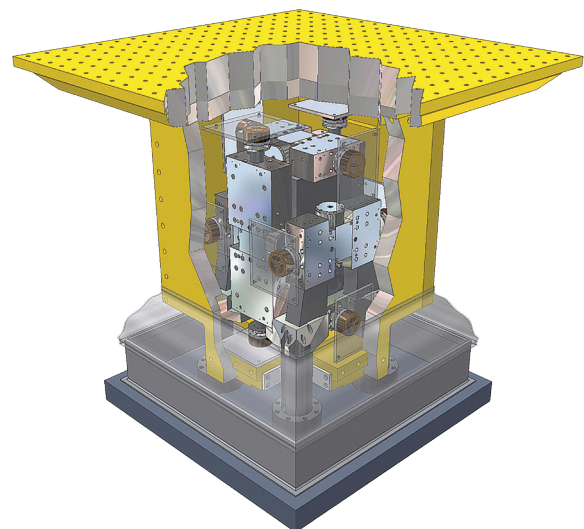
Figure 1. Team Cube 6 DOF Shaker System
