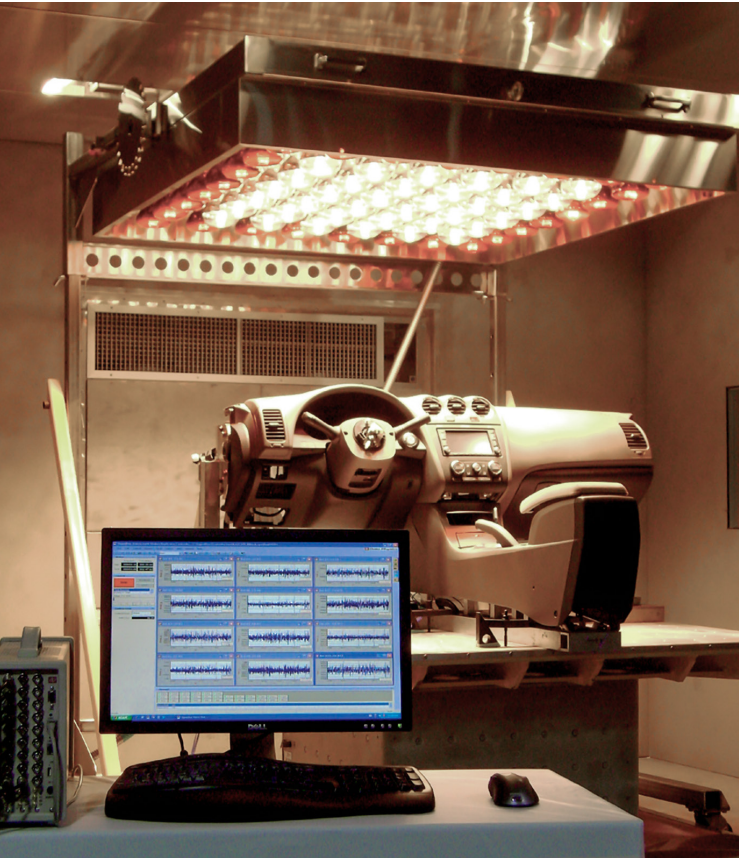
Figure 5. A Data Physics Matrix multi-DOF vibration controller runs a time waveform replication test on a Team Cube 6DOF shaker system for cockpit modules.
