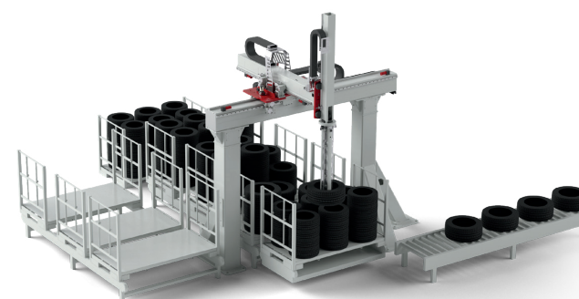
TIRE DE-PALLETIZER
