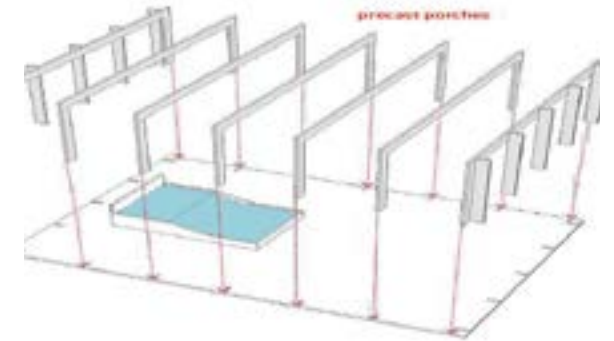
PRIMARY STRUCTURE
