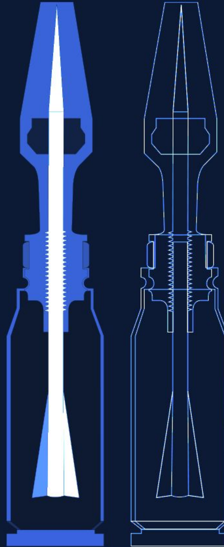
MK258 SWIMMER
