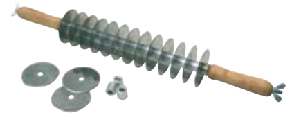
M1218 340 mm 21 knives (adjustable) Wooden handles Knives made out of stainless steel Inserts of 15 and 20 mm
