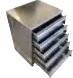
520mm(L)x430mm(W)x700mm(H)
