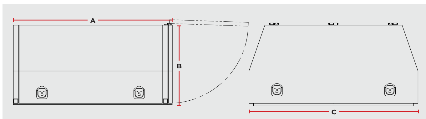
Norweld 3 Door Basic Canopy (2040mm Length) | Full-Time Deluxe Canopy Base (2040mm Length) | Ford Ranger
