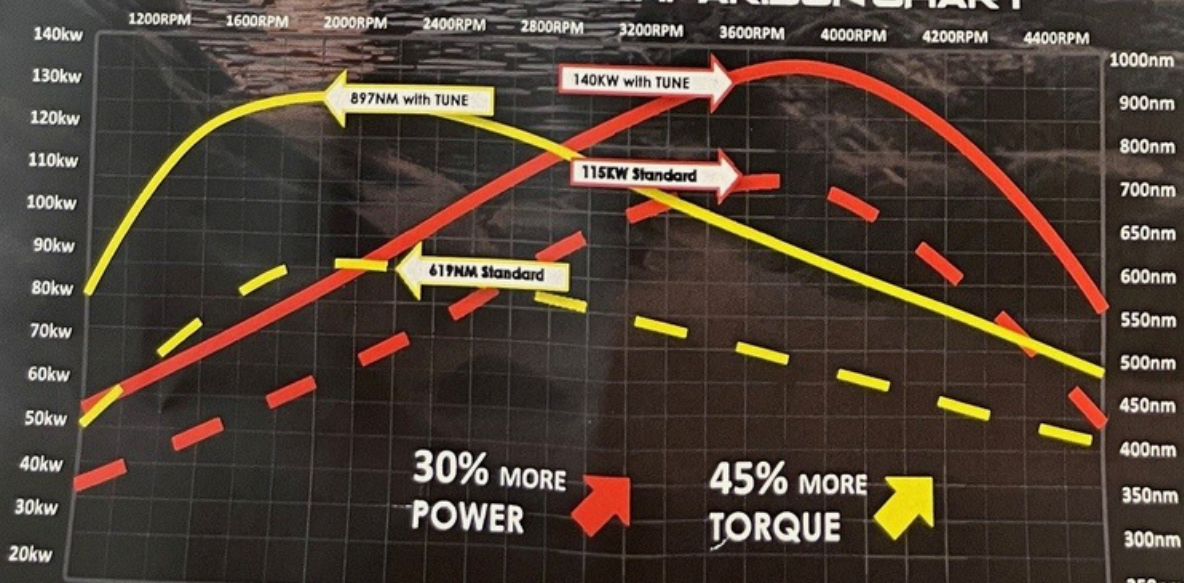
REAR WHEEL DYNO COMPARISON CHART
