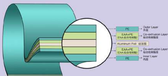
ABL (Aluminum Barrier Laminate) Tube 铝塑复合片材管
