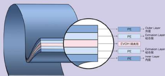
PBL (Plastic Barrier Laminate) Tube 全塑片材
