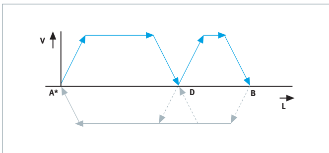
Basic profile for movement between two end positions: speed control with intermediate position
