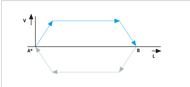
Basic profile for movement between two end positions: speed control without intermediate position
