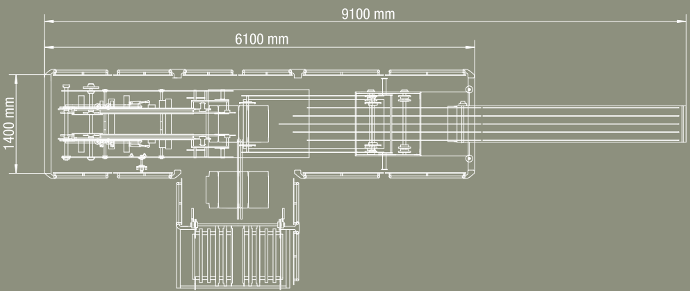
Top view of the machine type VP 501
