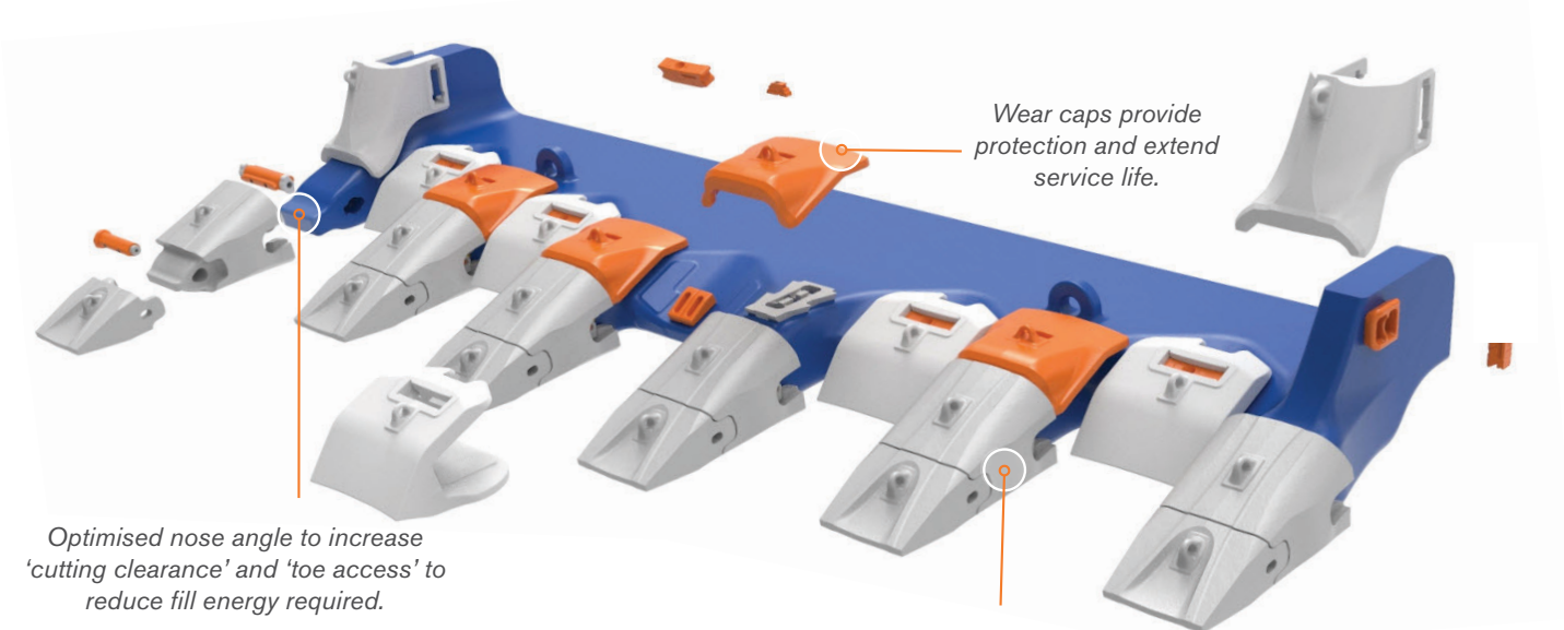
Improved adapter design to reduce nose maintenance from uneven wear and general nose peening.
