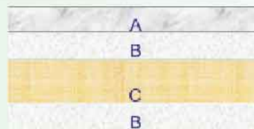
A: Resin coating layer (Satin, Luster, Silk) B: PE coating layer C: Base paper
