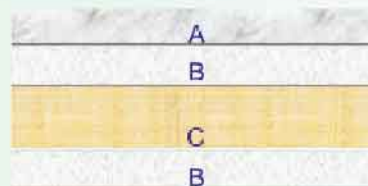
A: Resin coating layer (Glossy) B: PE coating layer C: Base paper
