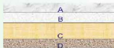
A: Ink receiving layer B: Base paper C: Adhesive layer D: Release paper
