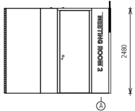
(A) Panel window with foil 488 x 2474 mm
