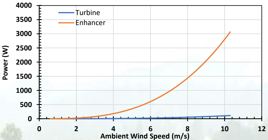
Plot of Power Vs Wind Speed (30/03/2021 AM)
