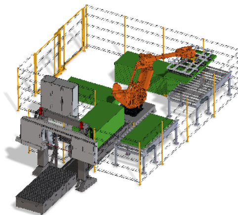
Horizontal band saw for cutting rigid foam with robot handling system
