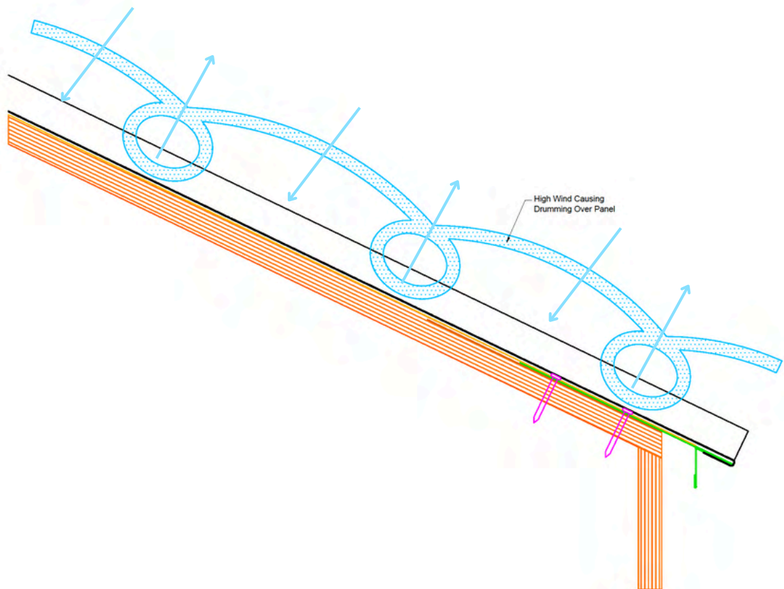
Figure 9.1 Wind drumming
