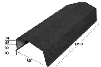
RECTANGULAR RIDGE
