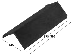
ANGLE TRIM
