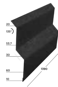
WALL FLASHING
