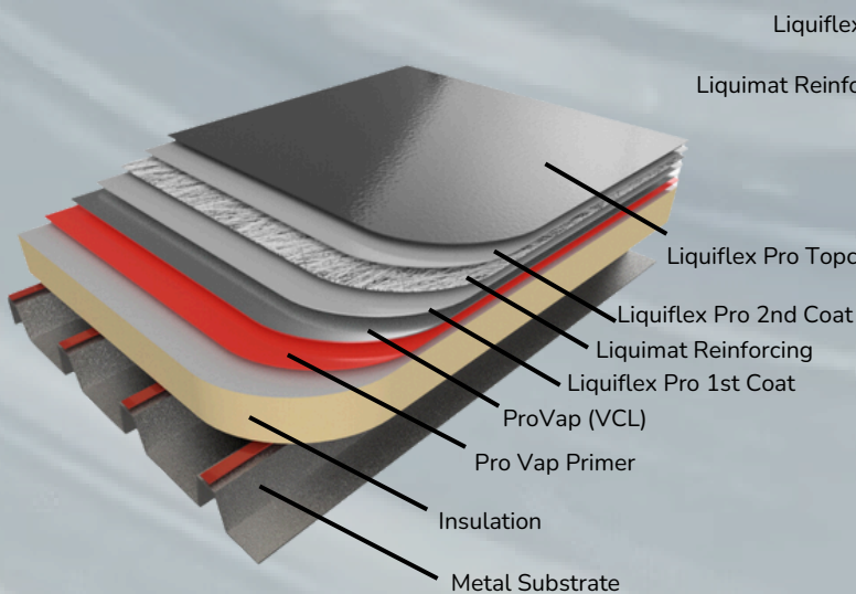
10 YEAR SYSTEM WITH A WARM ROOF BUILD UP
