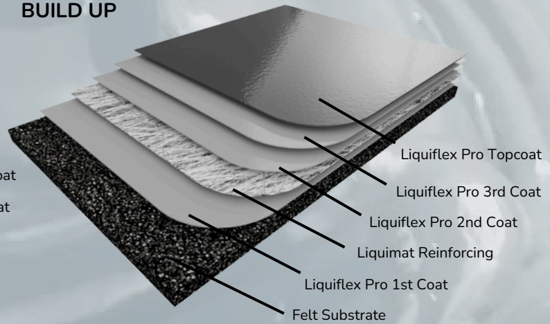
25 YEAR SYSTEM WITH A COLD ROOF BUILD UP
