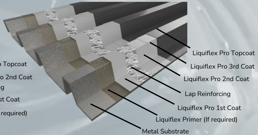
20 YEAR SYSTEM WITH A COLD ROOF BUILD UP
