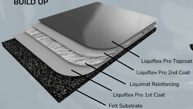
20 YEAR SYSTEM WITH A COLD ROOF BUILD UP
