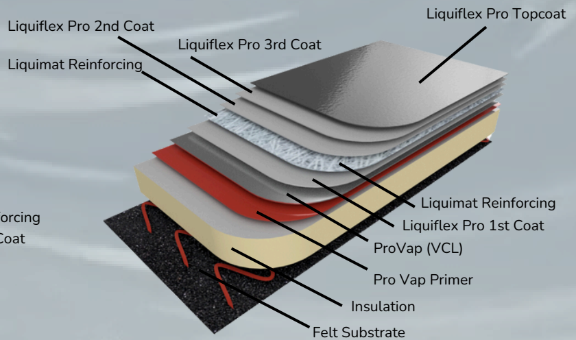
25 YEAR SYSTEM WITH A WARM ROOF BUILD UP
