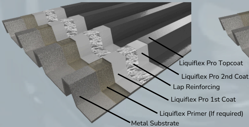
15 YEAR SYSTEM WITH A COLD ROOF BUILD UP
