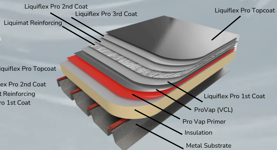
25 YEAR SYSTEM WITH A WARM ROOF BUILD UP
