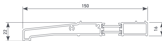
A-03089 - 150mm cill
