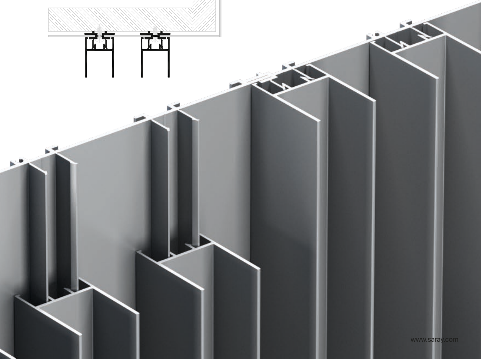
SVC05: the version that can be used individually with aluminium sheet between the cover profiles
