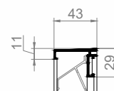
Surface-mounted wall louvre
