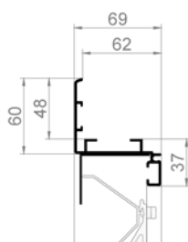
G 50Z Recessed wall louvre with flange
