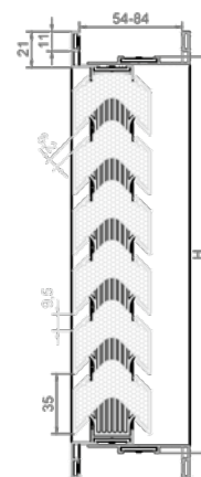
With counterframe 54-84 mm depth
