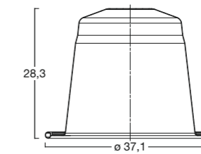
BARISTA Capsule Alu 2.0
