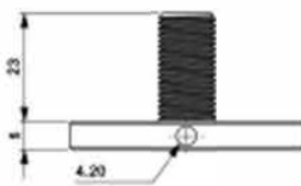
KT-ADJ-STAND-30 Adjustable Stand-Off, Satin or Mirror W 50mm x L 30mm 10-21.52mm Glass Duplex 2205
