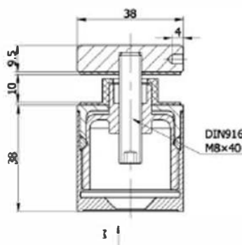
JK-1017-Black 316 Grade - Black Finish Stand Offs
