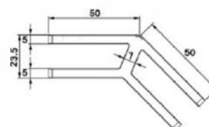
KLH10-STIFF-135 Duplex Stainless - Satin Finish 10-12mm 135 Degree Glass Stiffener
