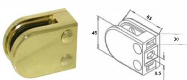
BR-10F Polished Brass (Gold) Glass Clamp 10mm Glass. 6/8/12mm Rubbers Also Available
