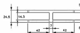
KLH10-STIFF-180 Duplex Stainless Steel - Satin Finish 10-12mm 180 Degree Glass Stiffener
