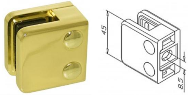
01.ZN.000.03.1000 Brass Glass Clamp Suitable for 6-10mm Glass 45 x 45mm Square
