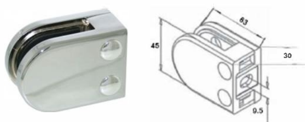
KLH10F-MIRROR Mirror Polished Glass Clamp 10mm Glass. 6/8/12mm Rubbers Also Available
