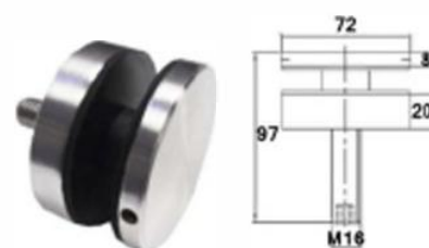
JK-1016 Solid Threaded Body - Flat Head M16 Removable Thread 304/316
