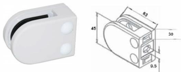
KLH10F-WHITE Powder Coated, White Glass Clamp 10mm Glass. 6/8/12mm Rubbers Also Available
