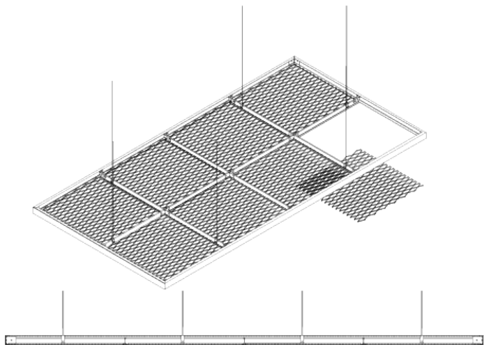
Mesh lay-in raft with exposed alumunium T grid
