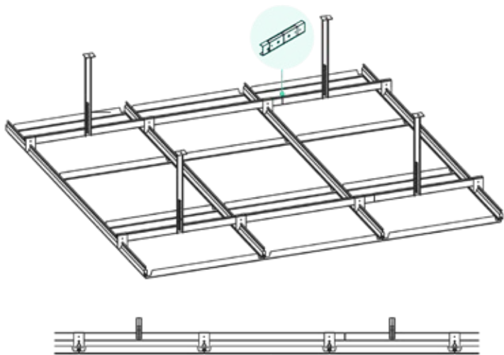
Clip-in metal panel with concealed grid
