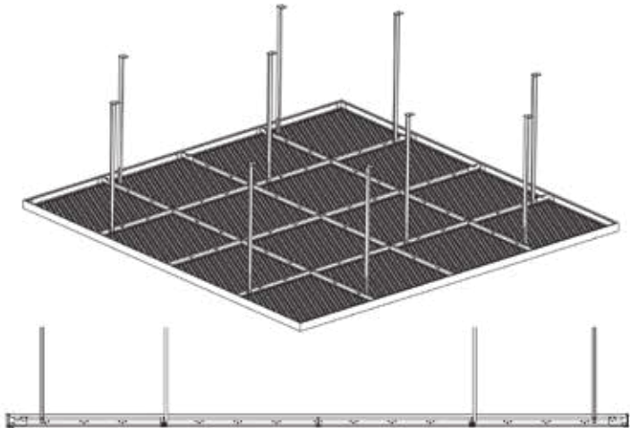
Mesh lay-in raft with exposed steel T-24 bar grid
