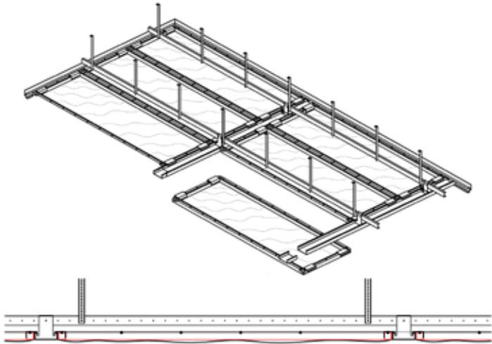
Lay-On Water-Ripple panels with exposed supporting service zone C-profiles
