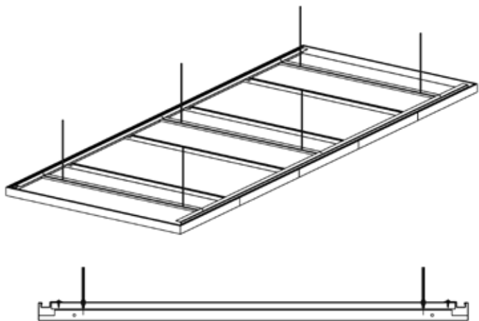
Hook-on shallow raft concealed grid
