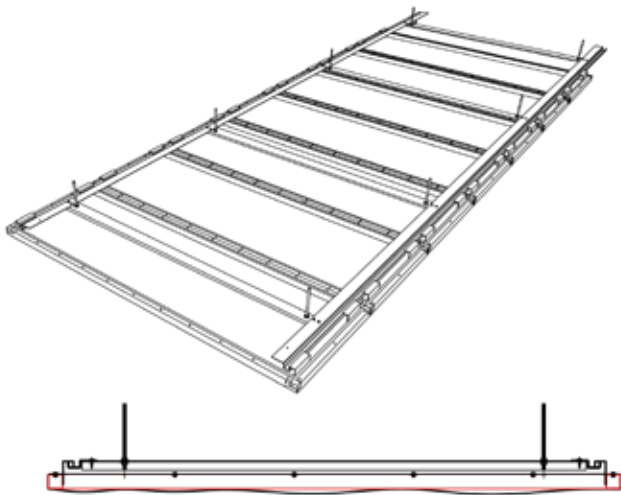
Water ripple hook-on shallow raft
