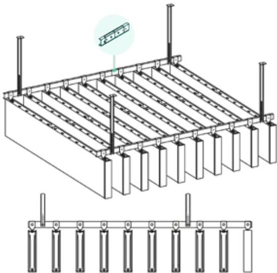
Acoustic baffle ceiling
