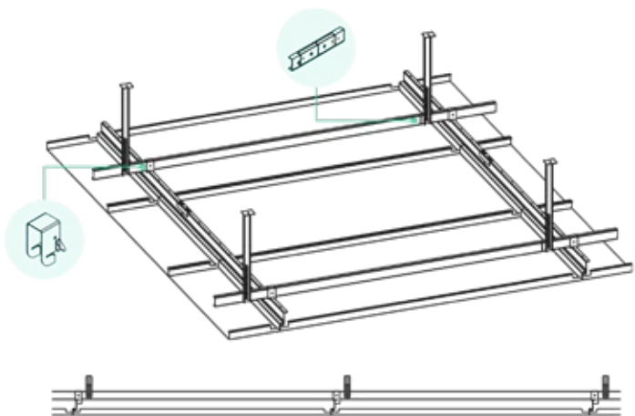
Hook-on Z-bar, concealed grid
