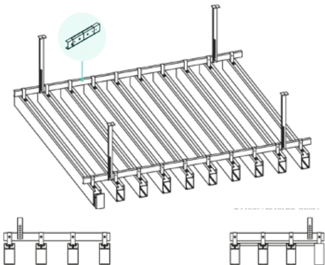
Acoustic aluminium linear slatted ceiling solution
