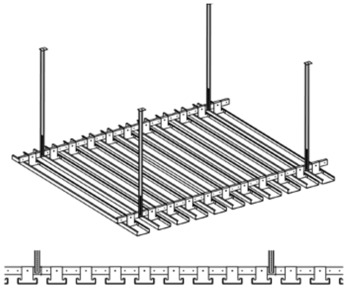
Linear exposed service zone C-profiles with nominal gaps
