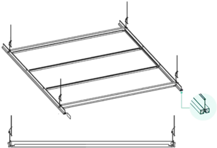
Lay-on metal panels supported on extruded one-way grid
