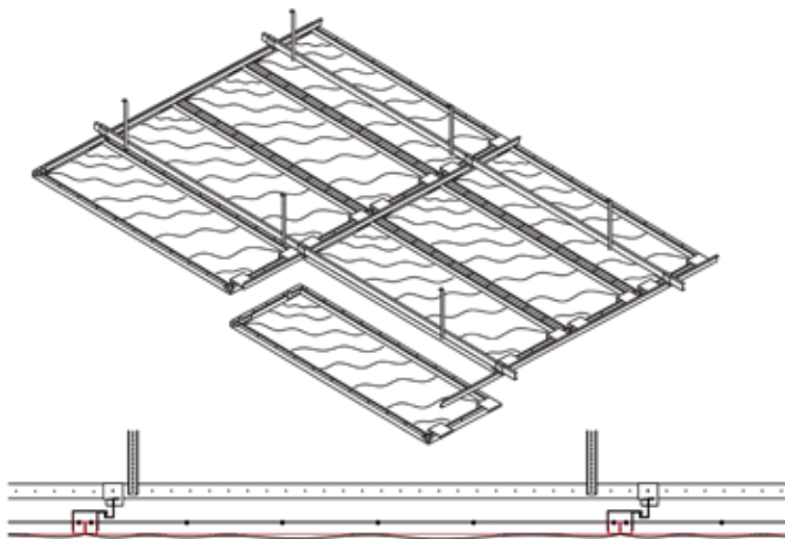
Water ripple hook-on Z-bar, concealed grid
