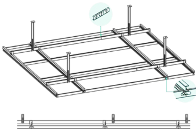
Hook-on H-bar, concealed grid
