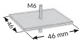
Fixing bracket
