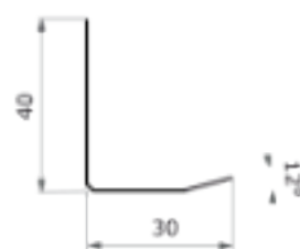
Perimetral "L" profile Cornice perimentrale a "L"
