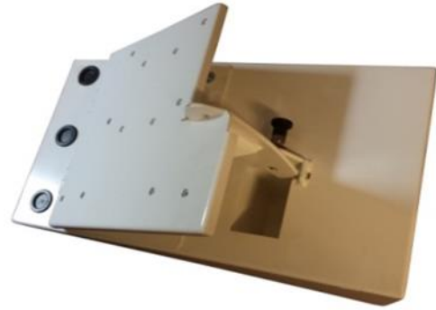
AP part no: DUC-0006-S AP Debrillator Bracket (to suit Life Pack 15)
