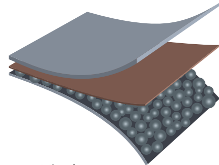
Schematic representation of a SARATOGA® compound
