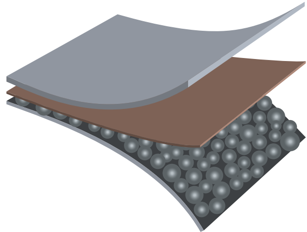
Schematic representation of a SARATOGA® compound fabric
