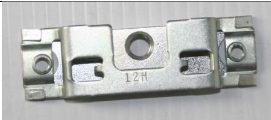
AP part no: MAC/515-0010-J Adjustable Cage Nut for Striker Pin (for use with MAC/515-0006-J Striker Pin) BIN Code 9821
