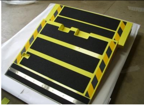
AP part no: REN-0014-S Renault MK2 Access Ramp Carcass
