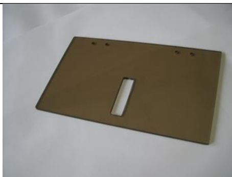
AP part no: GEN-0050-KV Smoked Acrylic Interior Locker Door Sliding 353x210mm with 1 Lock Cut-Out
