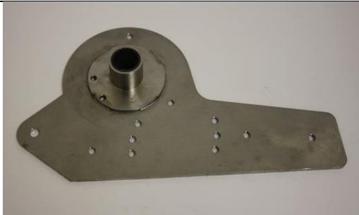
AP part no: RMP-0112-S Fiat Active 'P' Plate with Boss Attached
