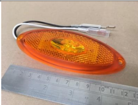
AP part no: GEN-0034-JL Mercedes Orange Side Marker Lamp LED 12v
