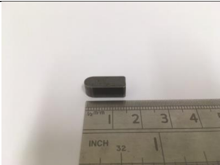
AP part no: RMP-0158-BO 16mm Key (Active axle) Bin No. 9171a
