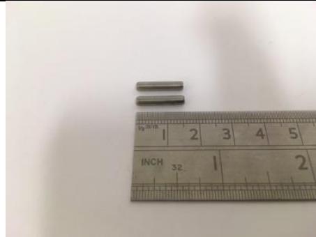
AP part no: RMP-0148-BO 2 x Clutch Sprocket Pins Fits 40mm and 50mm clutches
